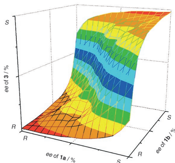
Figure 4. NLE in the Rh-catalyzed hydrogenation of 2 using mixtures of 1a and 1b , each with varying degrees of enantiopurity.
