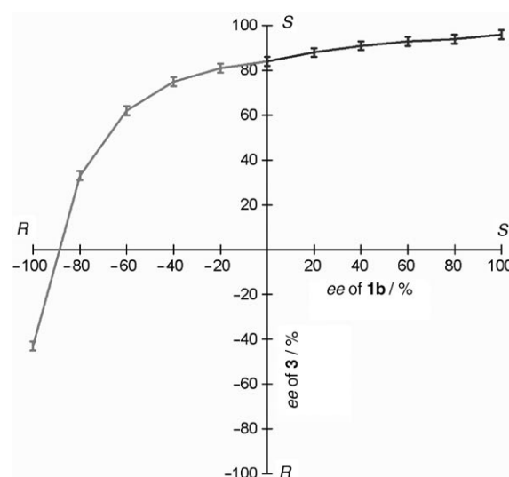
Figure 2. NLE in the Rh-catalyzed hydrogenation of 2 using enantiopure ( S )- 1a and 1b of varying enantiopurity.
