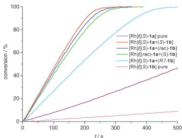
Figure 3. Relative rates of hydrogenation of 2 (Rh/ 2 = 1:5000, Rh/ 1 = 1:2, 1a/1b = 1:1, 1.3 bar H 2 , room temperature, CH 2 Cl 2 as the solvent).
