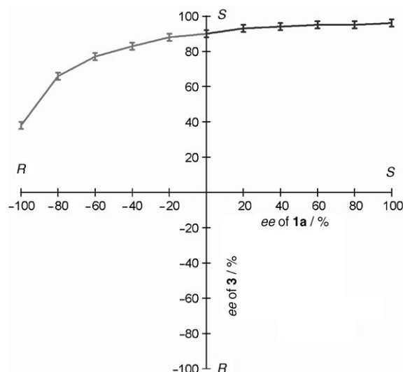
Figure 1. NLE in the Rh-catalyzed hydrogenation of 2 using enantiopure ( S )- 1b and 1a of varying enantiopurity.
